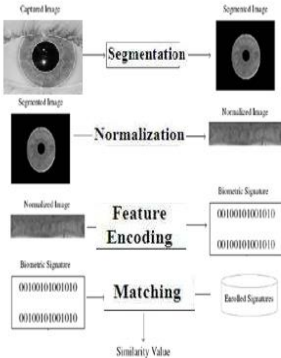
Figure 2: Stages of the Iris Detection Systems
