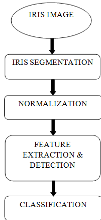
Figure 3: Methodology Flowchart
