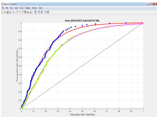
Figure 10: ROC curves for Sobel and Canny Edge Detectors
