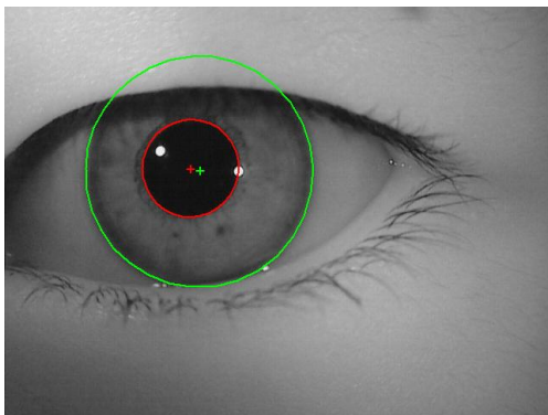
Figure 4: Segmented Image
