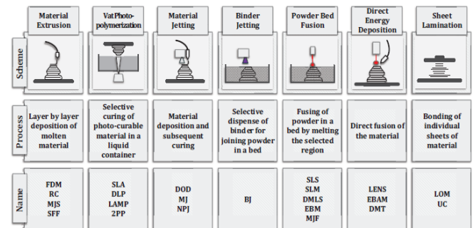
Fig. 3 Categorization of AM processes in the current state-of-the-art [12].
