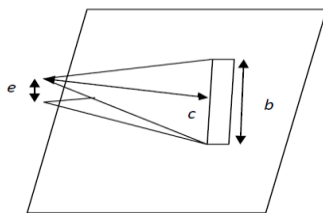
Fig.2(a): Delta wing vortex generator
