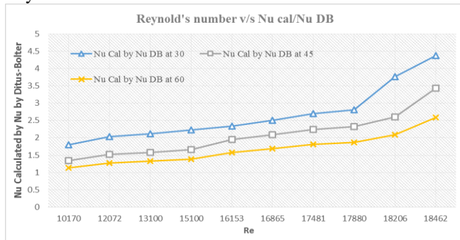
Graph 3: Re v/s Nu cal /Nu DB
