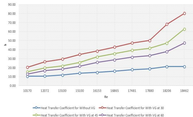
Graph 1: Re v/s h
