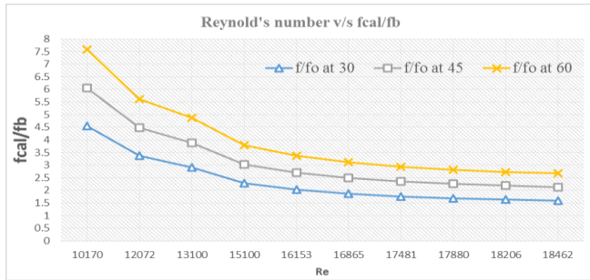
Graph 2: Re v/s fcal/fb
