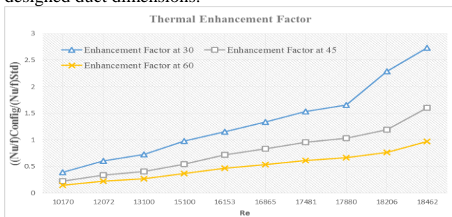
Graph 4: Thermal Enhancement Factor
