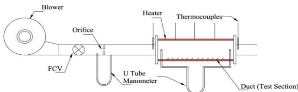
Fig.1: Experimental Setup
