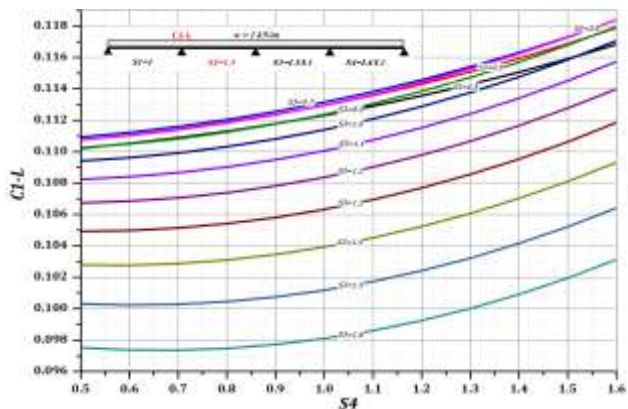
Chart 21: Coefficient C1-L for 4-spans, S2 (1.5), S3 & S4 (0.5-1.6)
