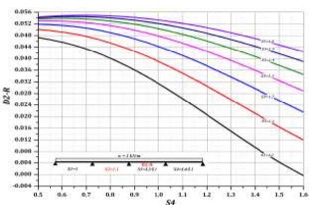
Chart 84: Coefficient D2-R for 4-spans, S2 (1.1), S3 (1.0-1.6) & S4 (0.5-1.6)
