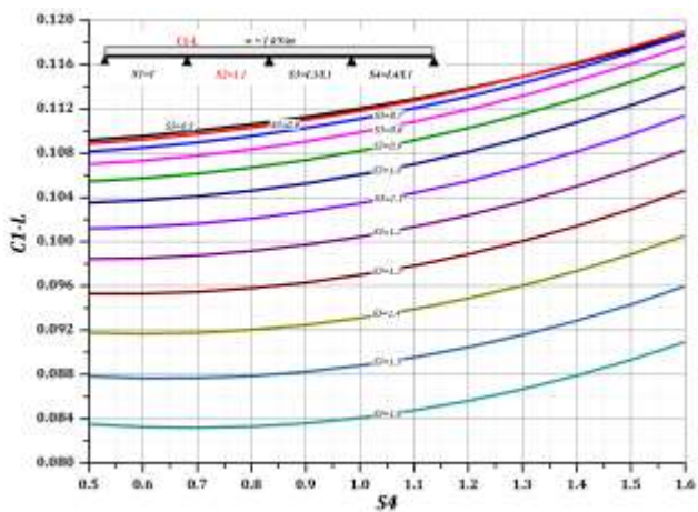
Chart 17: Coefficient C1-L for 4-spans, S2 (1.1), S3 & S4 (0.5-1.6)
