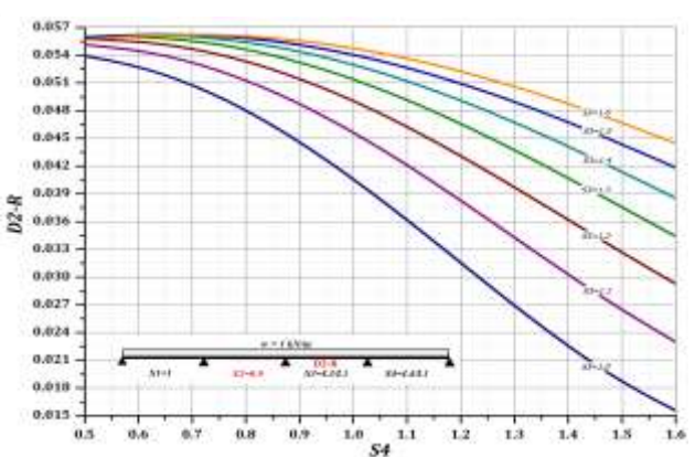
Chart 80: Coefficient D2-R for 4-spans, S2 (0.9), S3 (1.0-1.6) & S4 (0.5-1.6)
