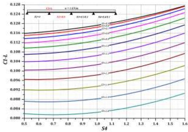
Chart 15: Coefficient C1-L for 4-spans, S2 (0.9), S3 & S4 (0.5-1.6)
