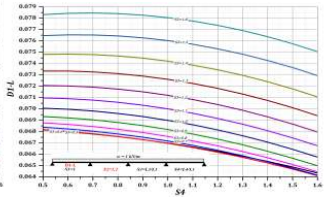
Chart 54: Coefficient D1-L for 4-spans, S2 (1.2), S3 & S4 (0.5-1.6)
