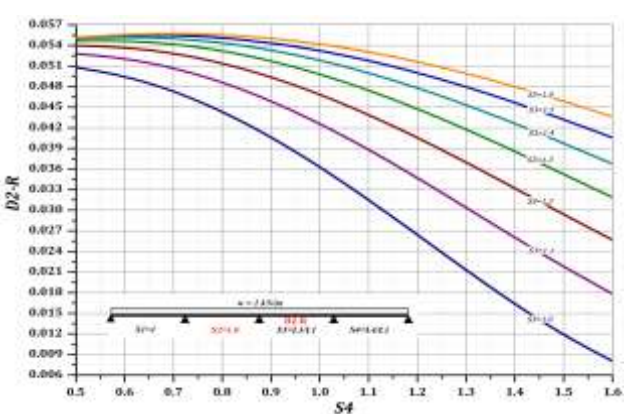
Chart 82: Coefficient D2-R for 4-spans, S2 (1.0), S3 (1.0-1.6) & S4 (0.5-1.6)
