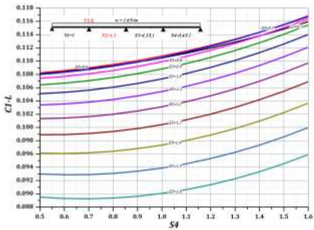
Chart 19: Coefficient C1-L for 4-spans, S2 (1.3), S3 & S4 (0.5-1.6)
