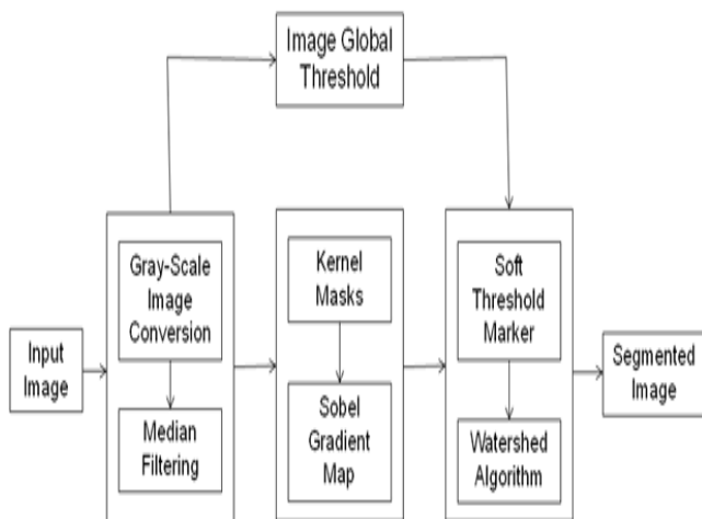
Fig. 6 The basic components of the proposed watershed based segmentation framework.
