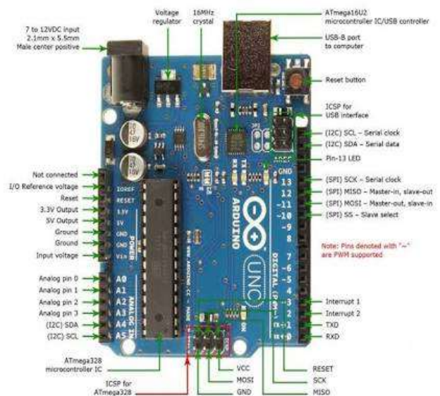
Figure 1. Arduino Uno with AT Mega microprocessor
